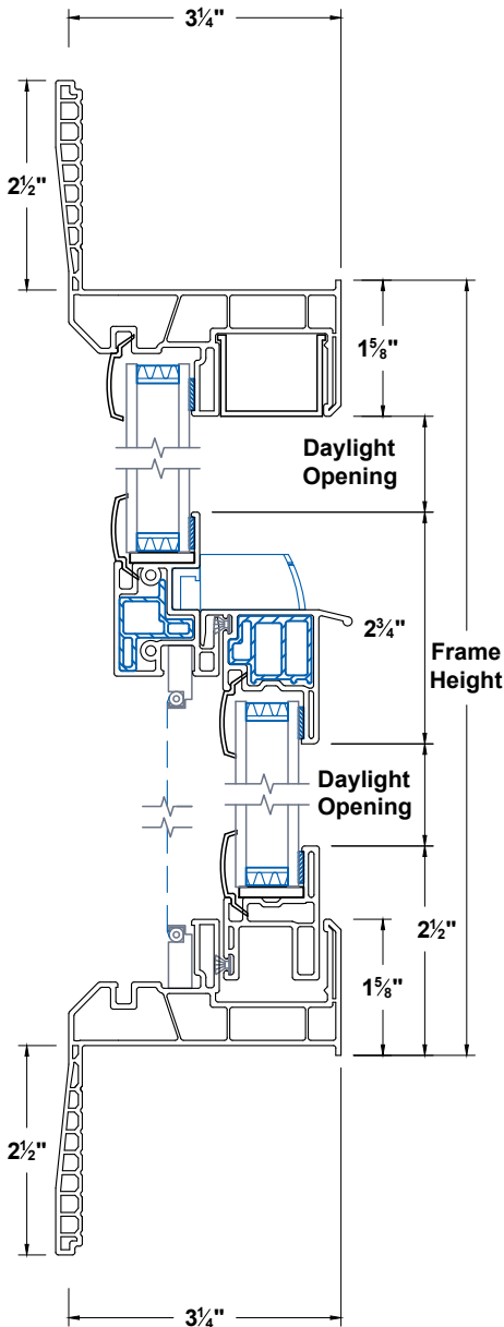
Head & Sill
