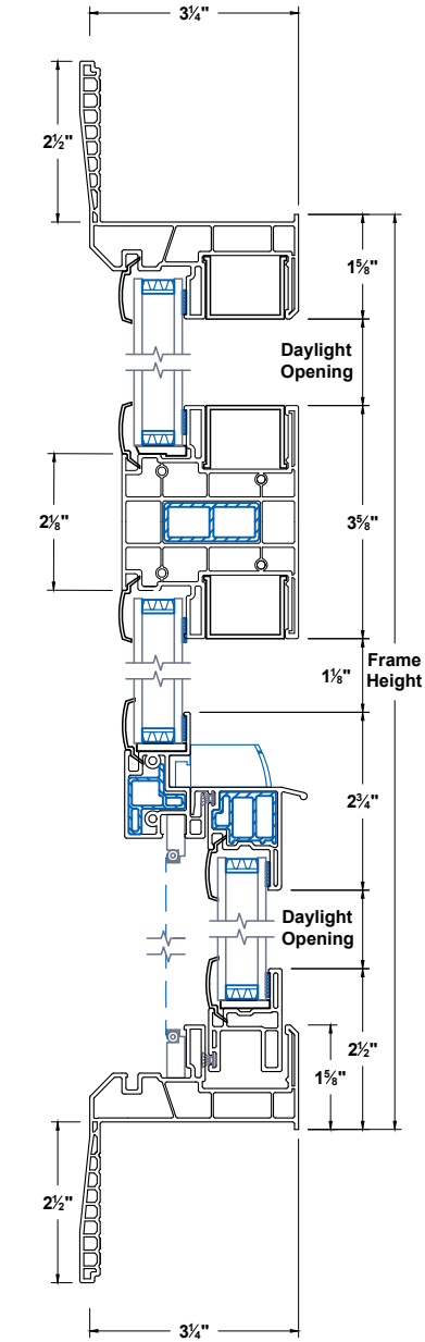
Head & Sill
