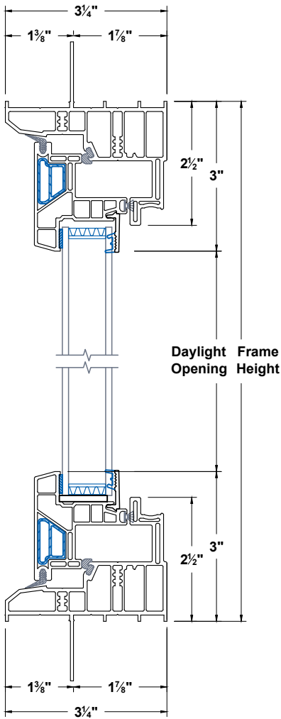
Head & Sill
