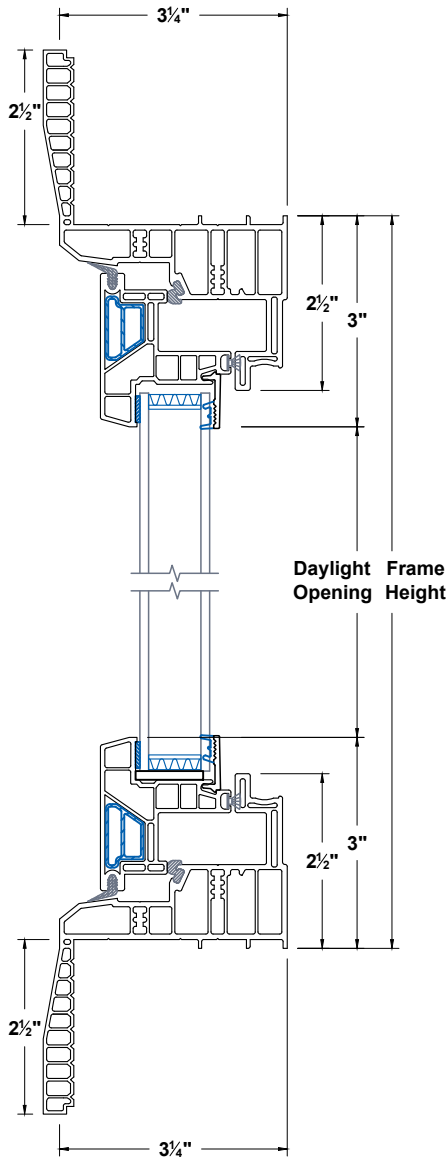
Head & Sill
