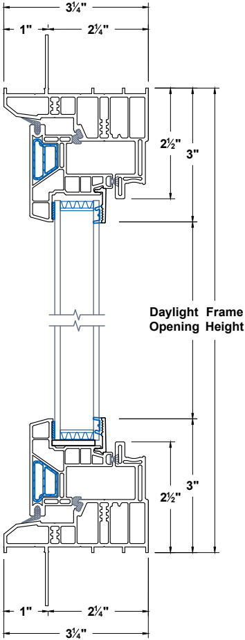
Head & Sill
