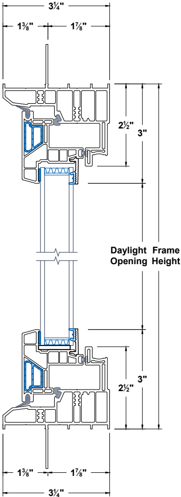
Head & Sill
