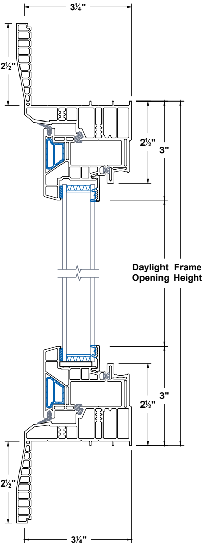
Head & Sill
