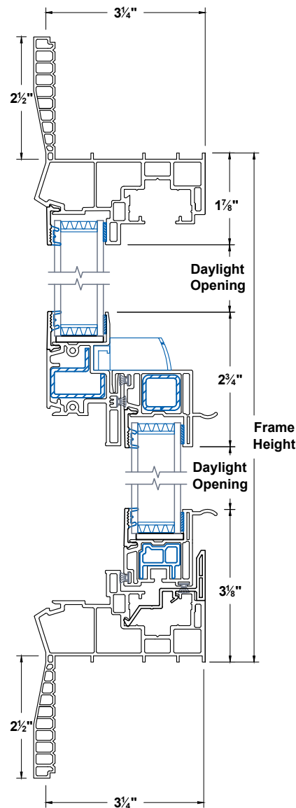
Head & Sill
