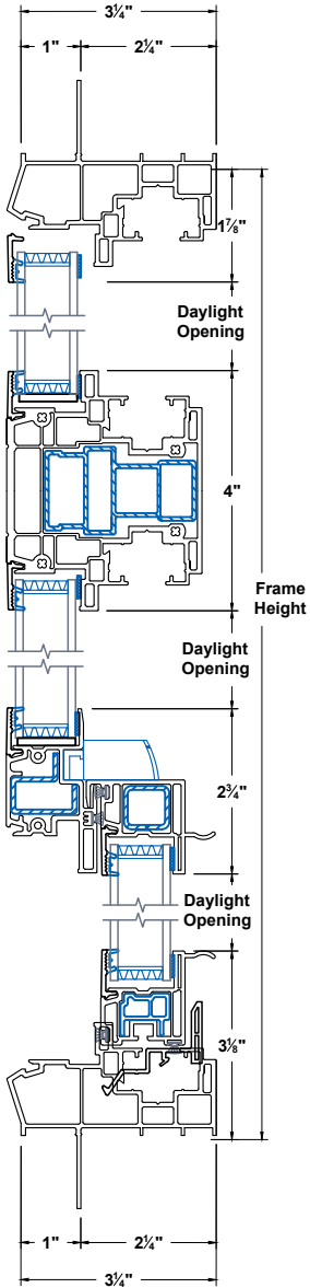
Head & Sill
