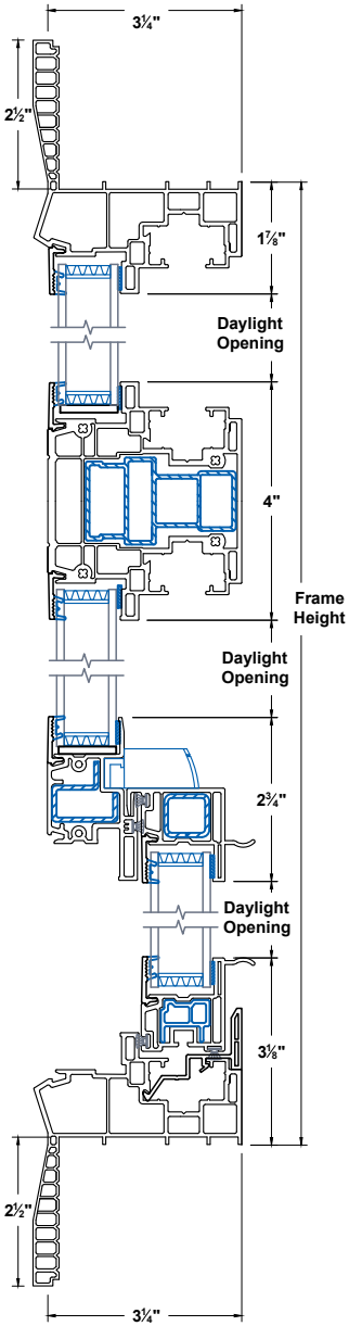
Head & Sill
