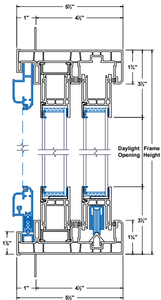
Head & Sill
