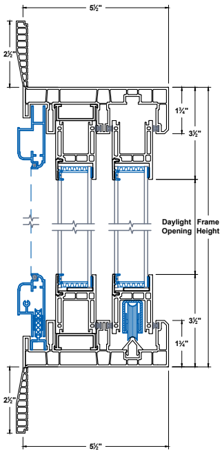
Head & Sill
