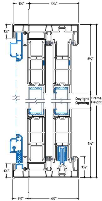
Head & Sill
