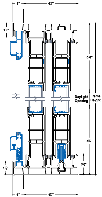
Head & Sill
