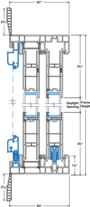
Head & Sill
