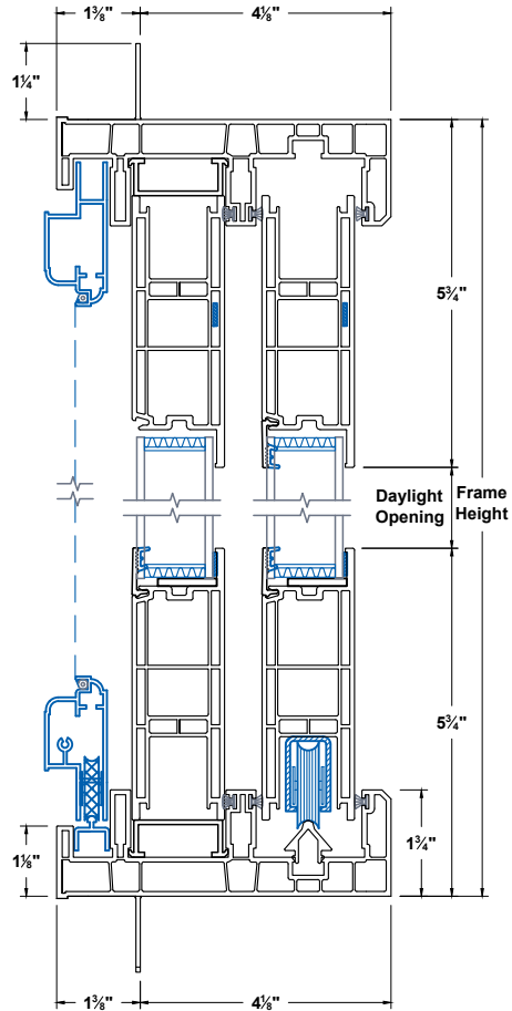
Head & Sill
