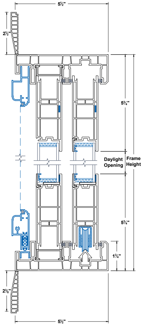
Head & Sill
