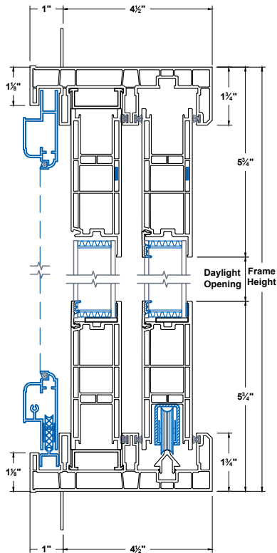
Head & Sill
