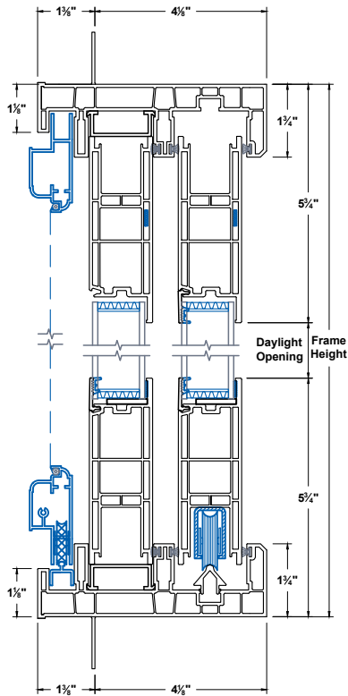
Head & Sill
