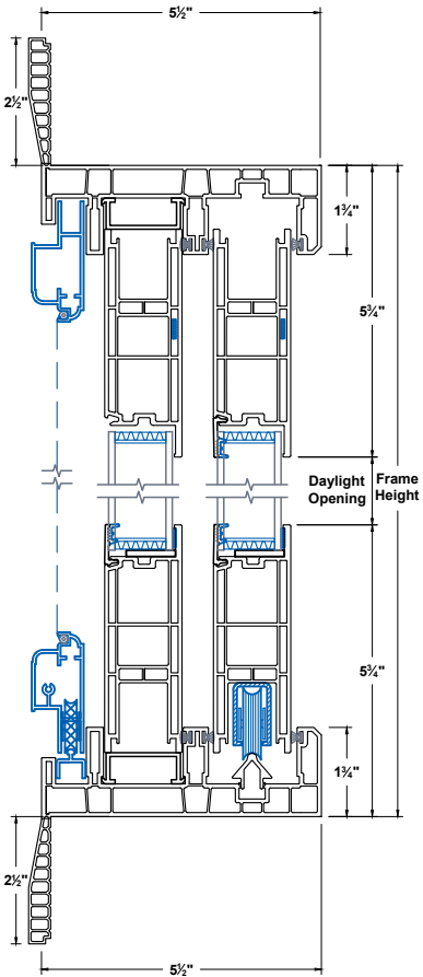
Head & Sill
