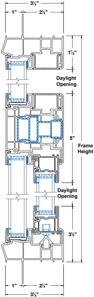
Head & Sill
