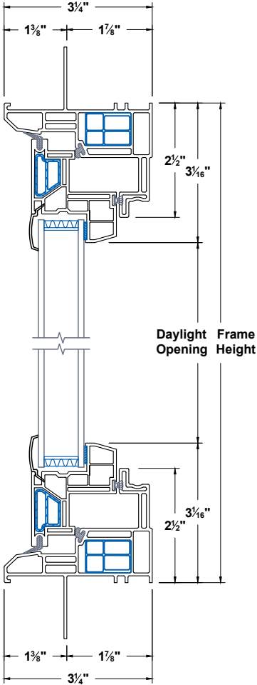
Head & Sill
