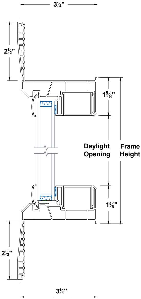
Head & Sill
