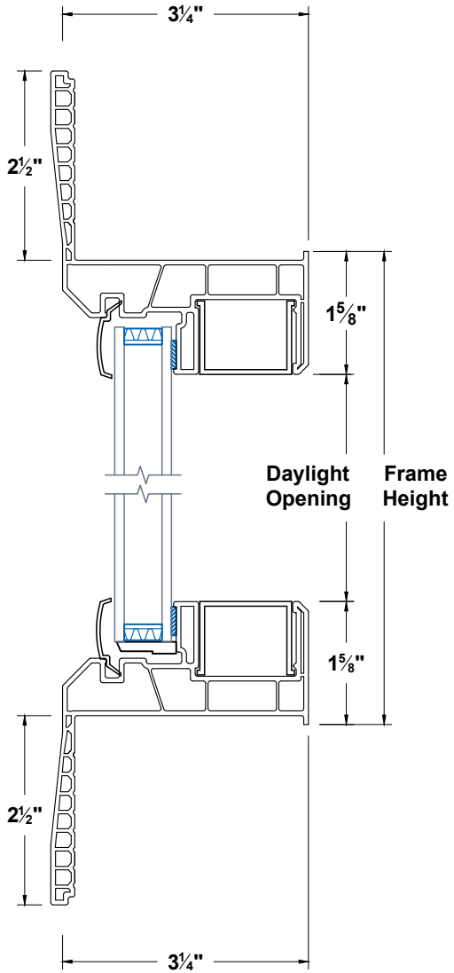
Head & Sill
