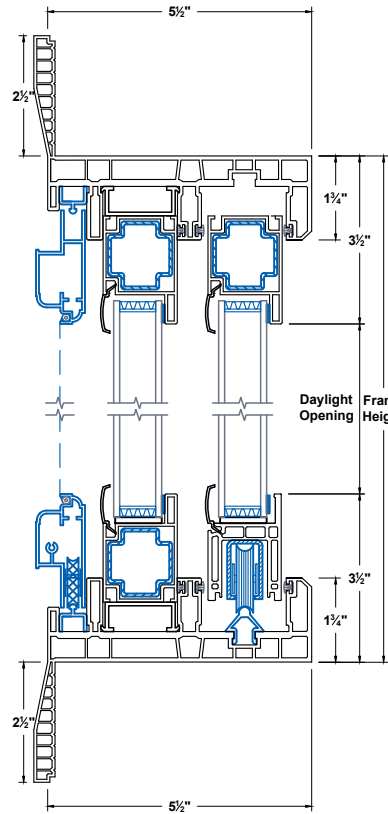
Head & Sill
