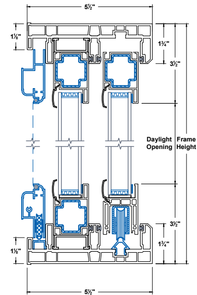
Head & Sill
