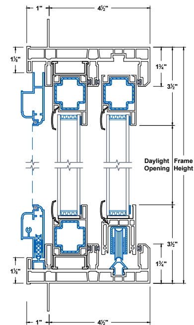
Head & Sill
