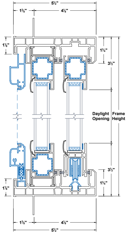
Head & Sill
